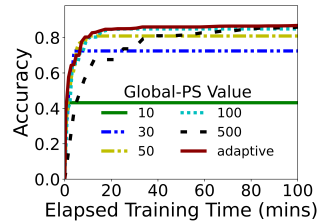
Figure 17: Adaptive vs Fixed. Model:DistilBERT. Dataset:AGNews
