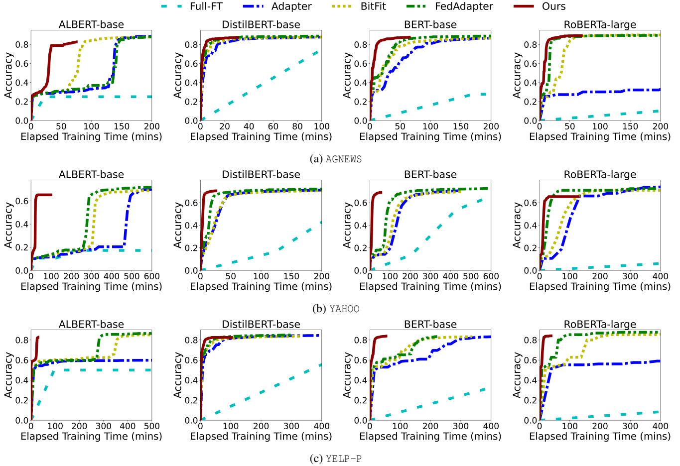
Figure 10: Overall Performance of FwdLLM and baselines. Processor: NPU for FwdLLM and CPU for others.
