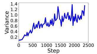
Figure 8: Gradient Variance through training.
