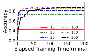
Figure 7: Optimal Global-PS varies across training.
